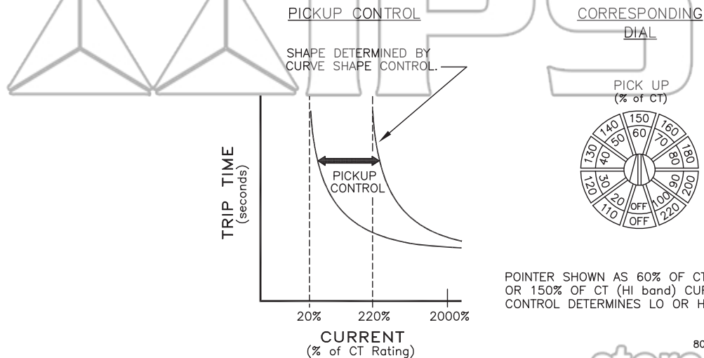
FIGURE 3–2: Phase Pickup Setting
