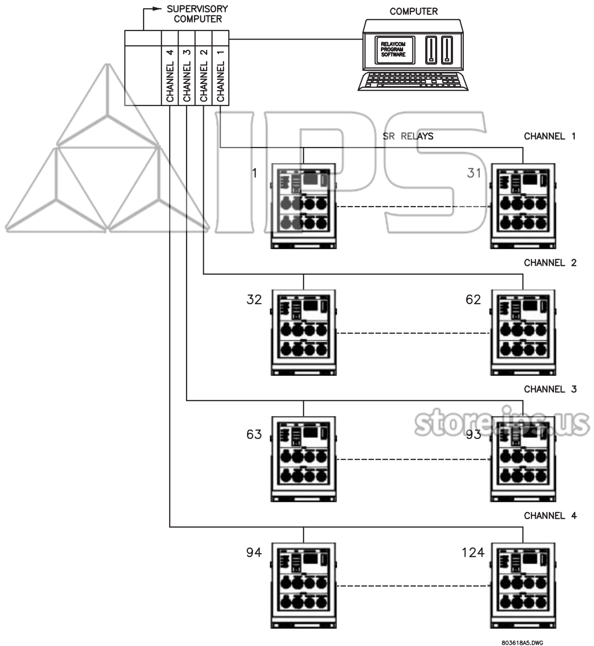
FIGURE 2-13: 4 Channel, 124 Relay System
