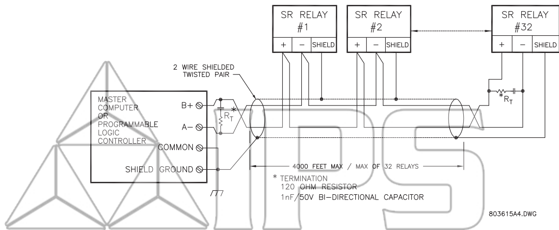
FIGURE 2-12: RS485 Termination
