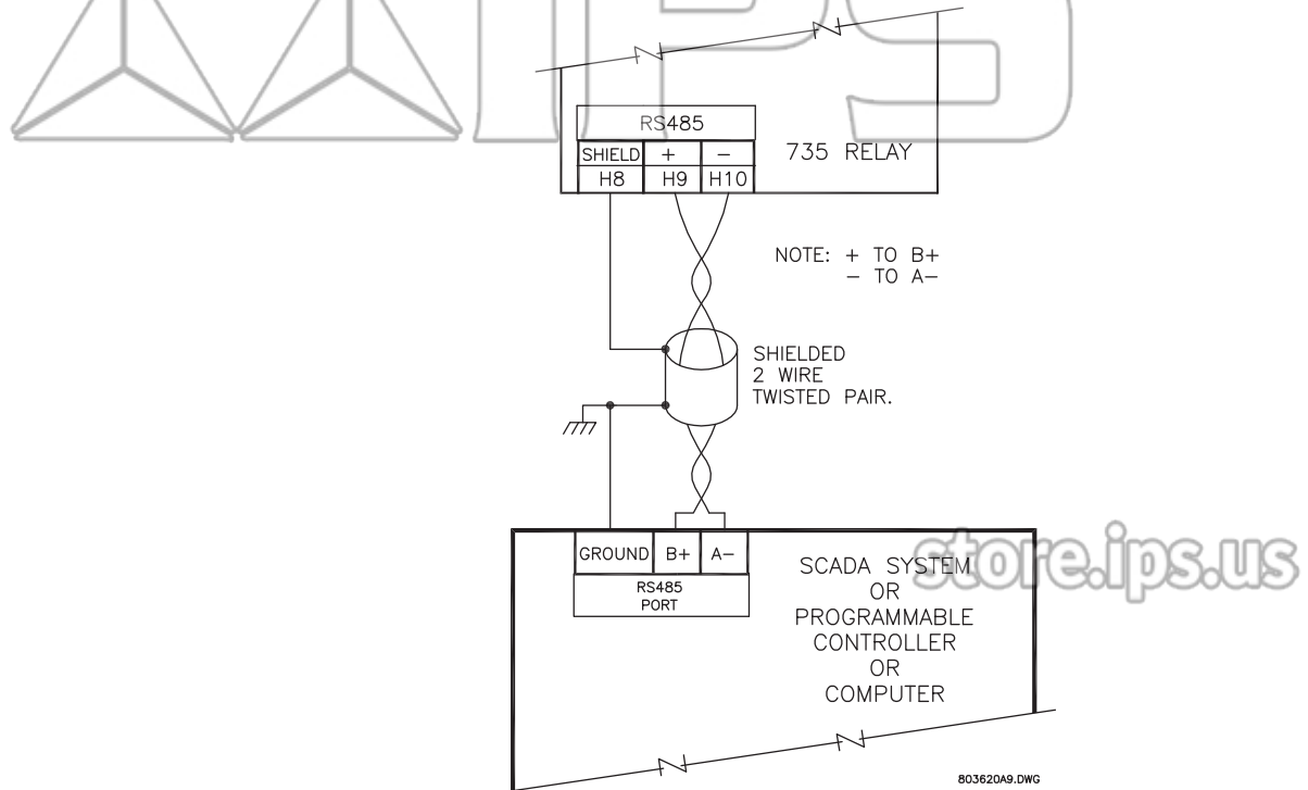
FIGURE 2-11: RS485 Connection
