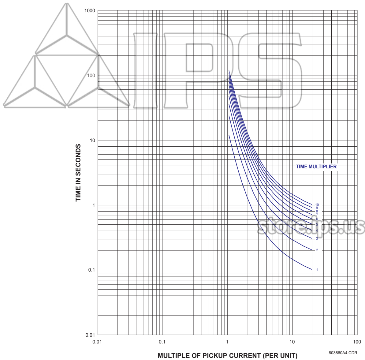
FIGURE 5-3: ANSI Very Inverse Curves
