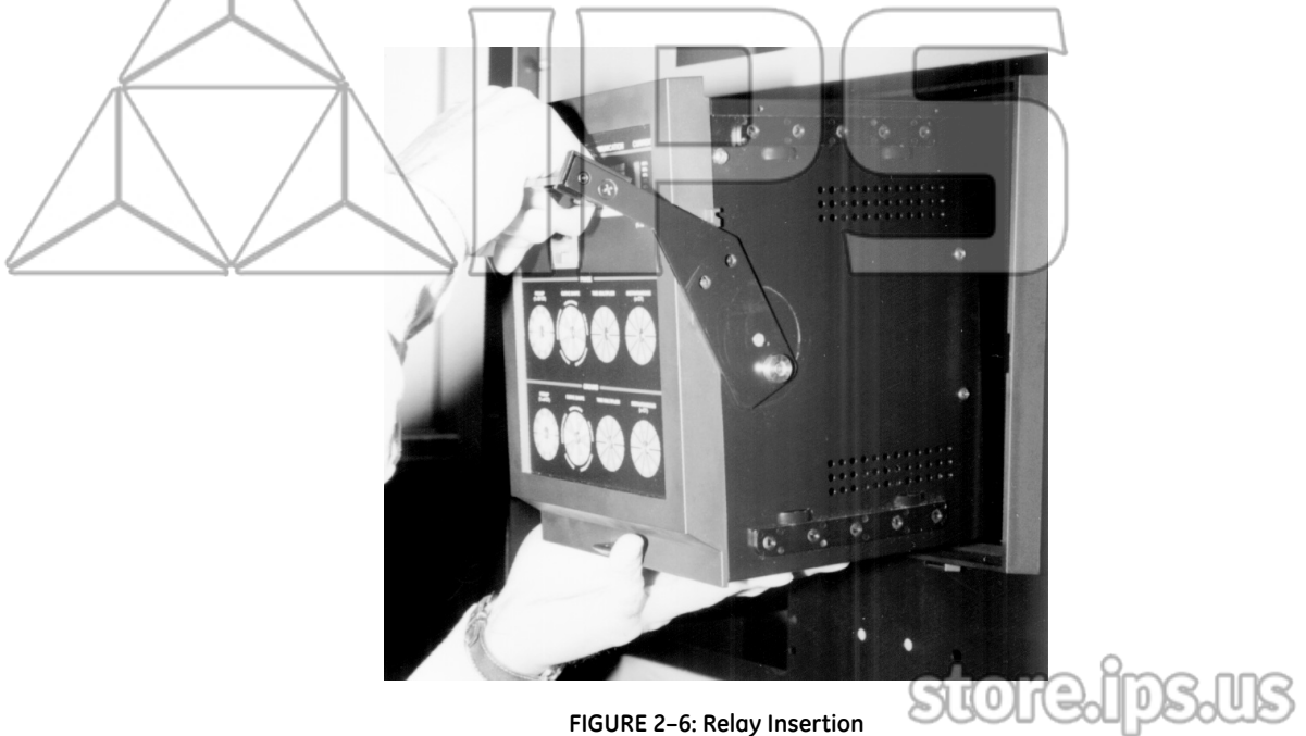
FIGURE 2-6: Relay Insertion
