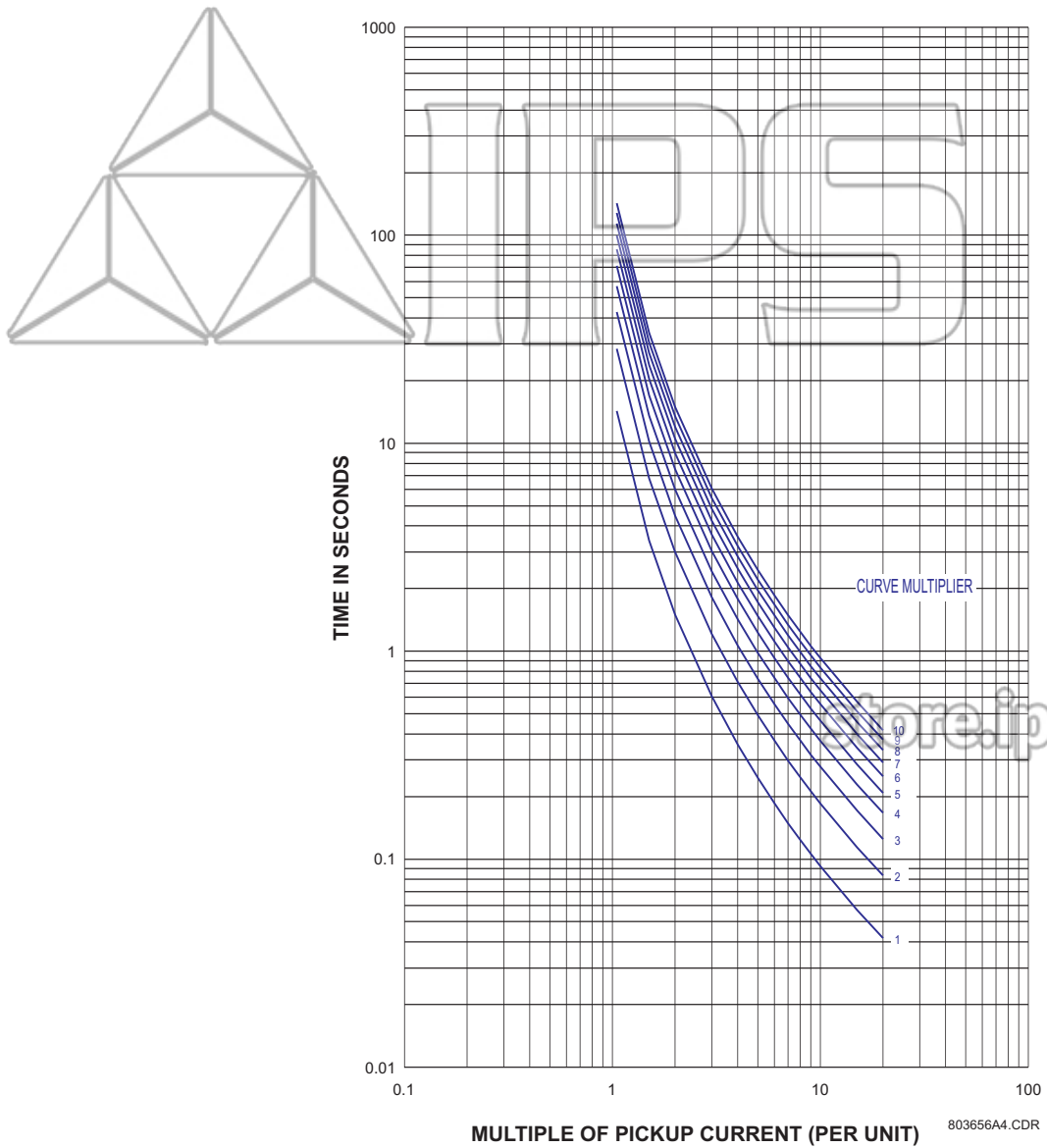
FIGURE 5-9: IAC Extremely Inverse Curves
