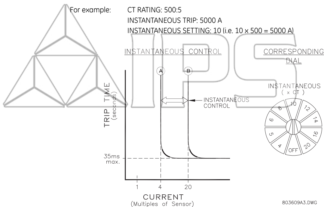
FIGURE 3-5: Phase Instantaneous Trip Setting
