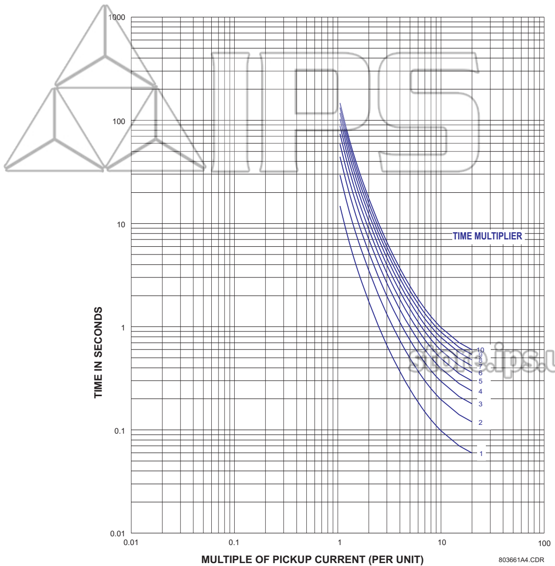
FIGURE 5-4: Ansi Extremely Inverse Curves
