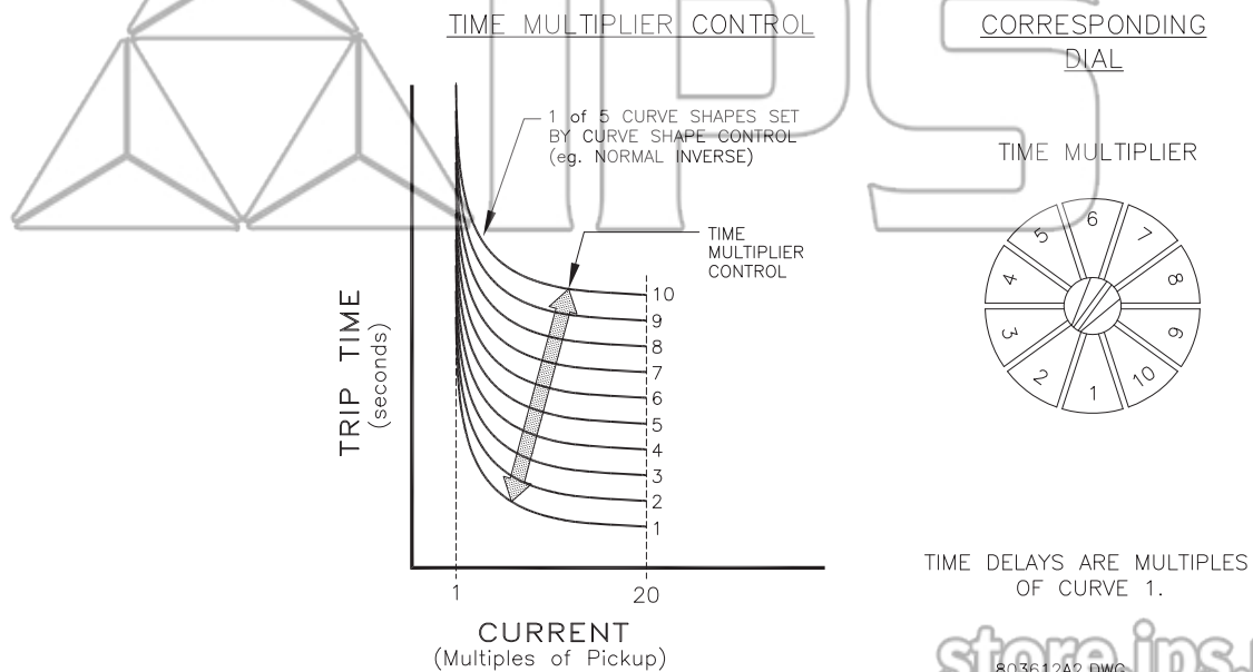
FIGURE 3-8: Ground Time Multiplier Setting
