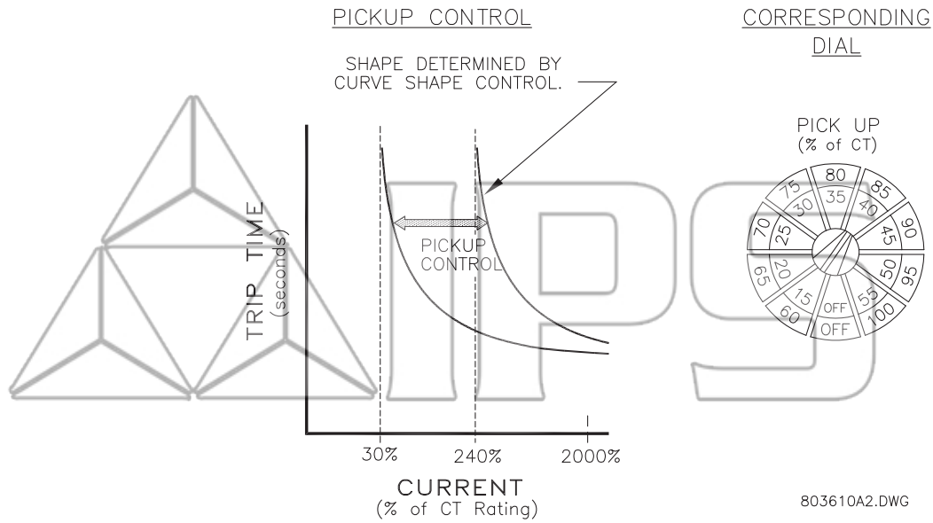
FIGURE 3-6: Ground Time Pickup Setting
