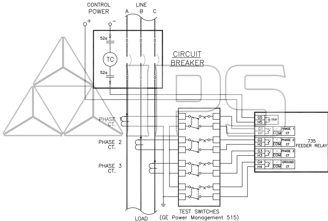
RESIDUAL RELAY CONNECTION
