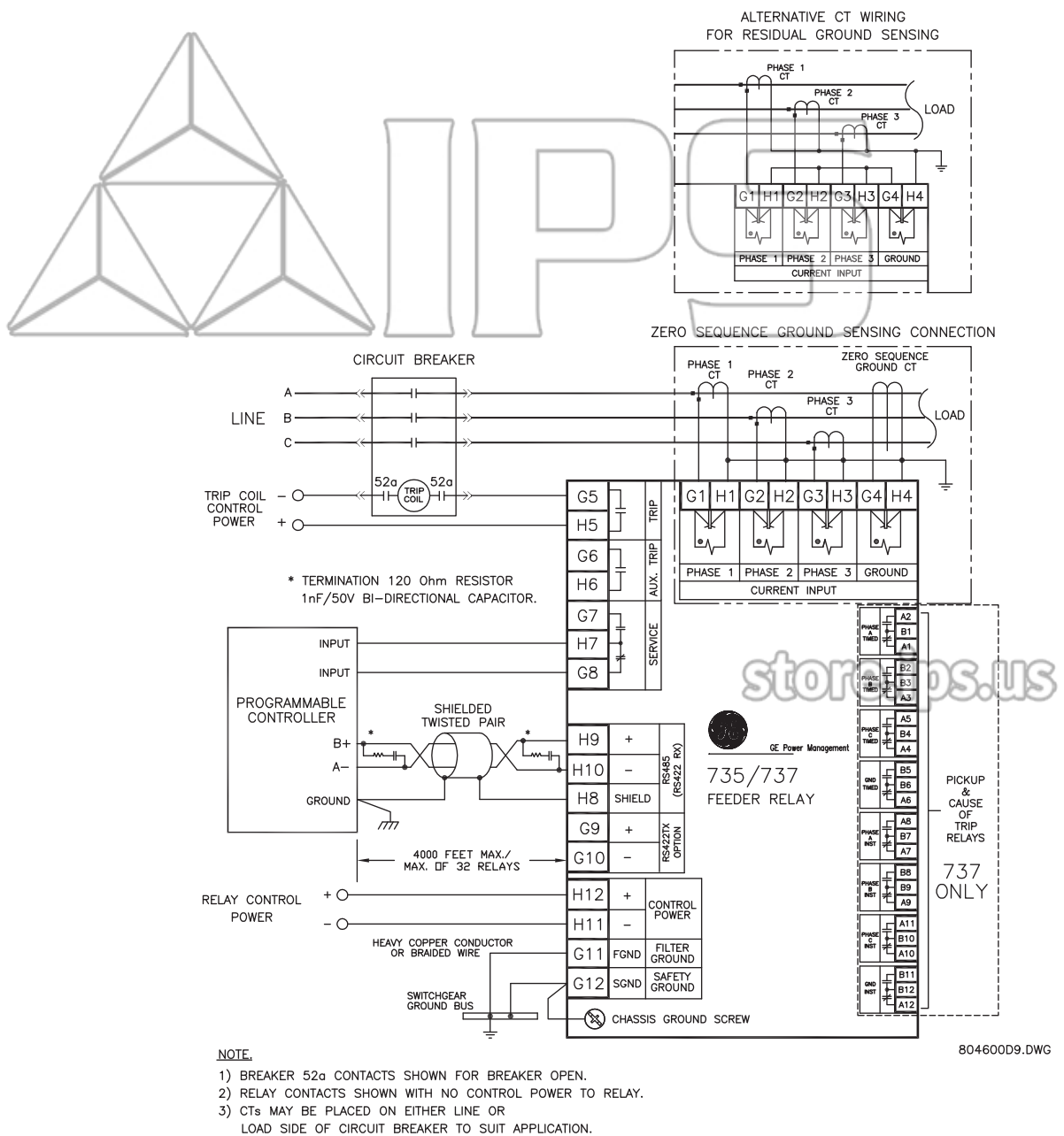
FIGURE 2-8: Typical Wiring Diagram
