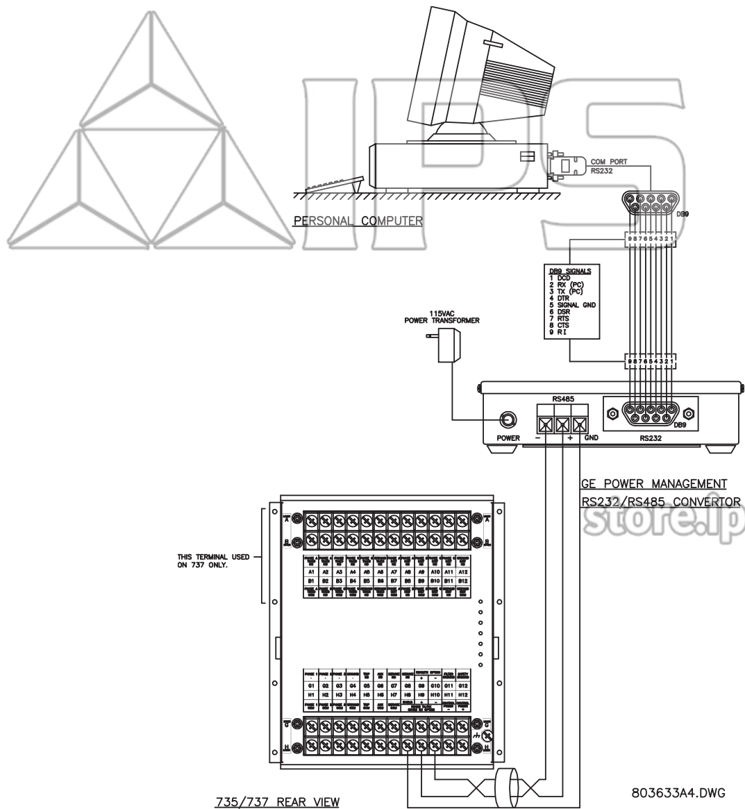
FIGURE 2-14: RS232/485 Converter
