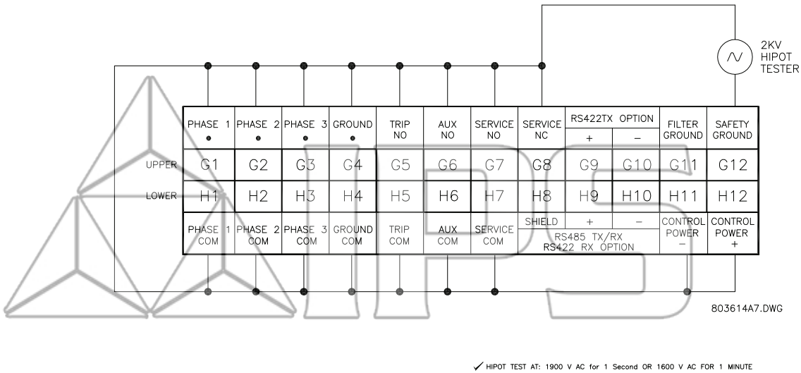
FIGURE 2-15: HI-POT Testing Connections
