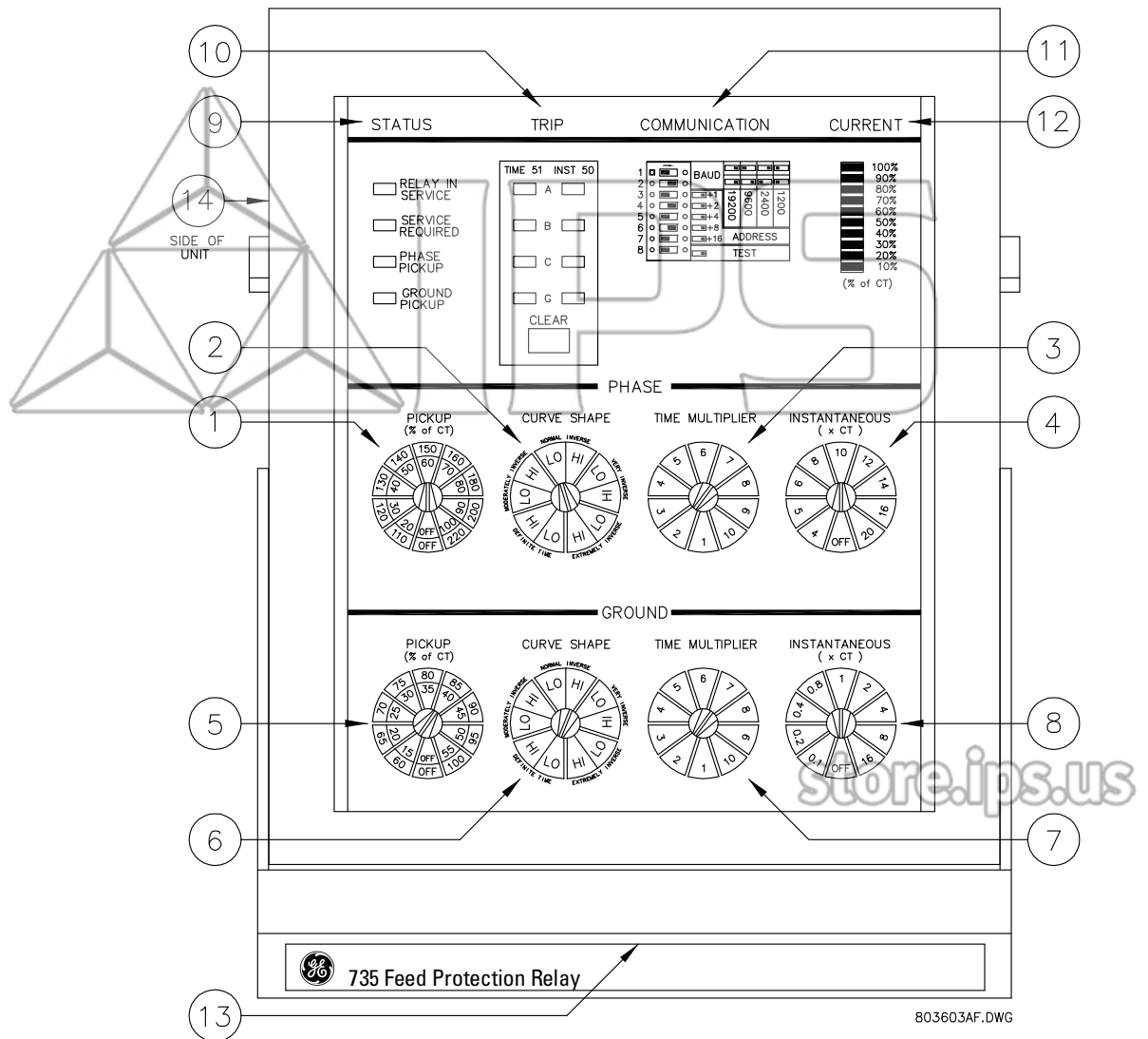
FIGURE 3-1: Front Panel Controls and Indicators
