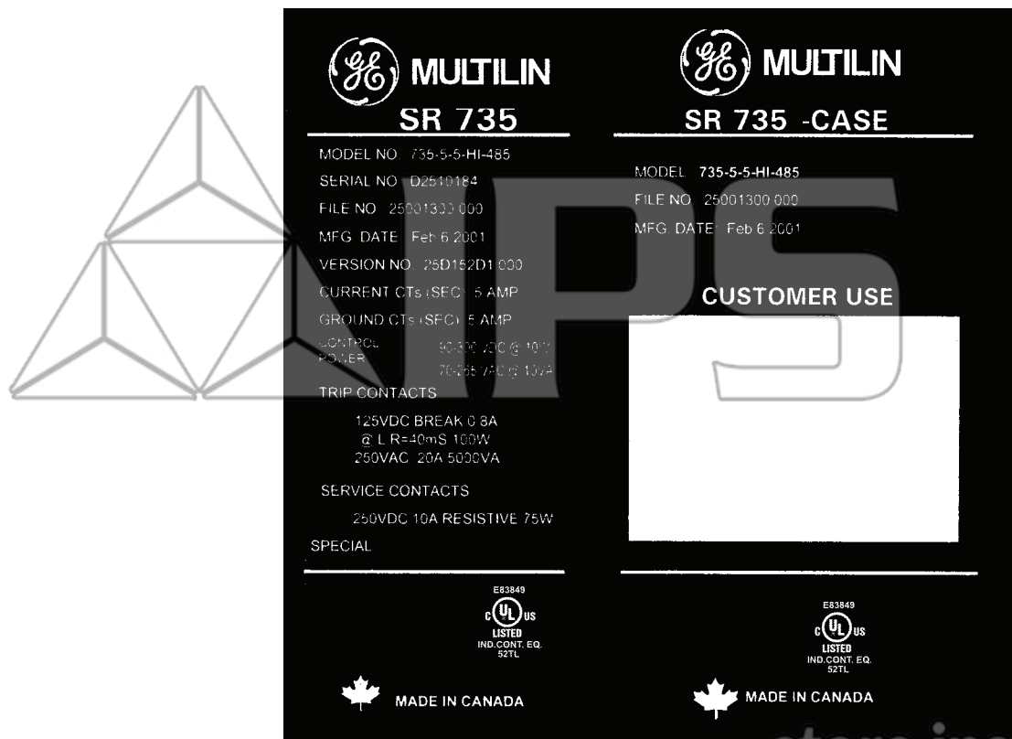
FIGURE 2-7: 735 Labels
